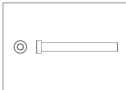
46. Bolt, 3/8-16 x 3-1/4" (83mm) socket head QTY 2
