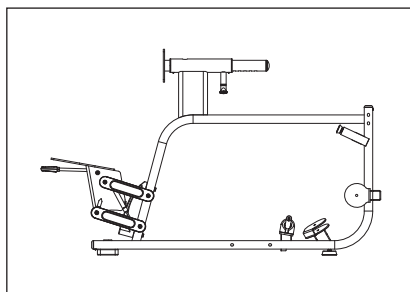
1. SR main frame QTY 1
