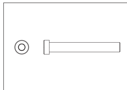
7. Bolt, 3/8-16 x 2-3/4" (70mm) socket head QTY 4
