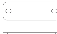
11. Plate, 50 x 155 x 4 mm QTY 1
