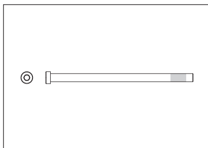
5. Bolt, 3/8-16 x 6-1/4" (159mm) socket head W/NP QTY 4
