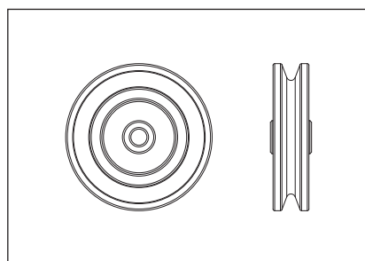
49. Pulley, 3.5"OD x 25 QTY 1
