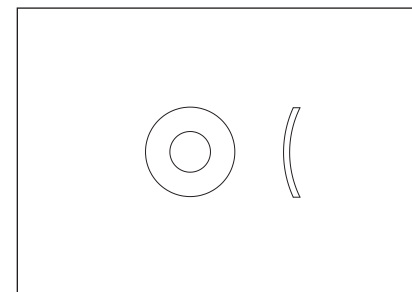
4. Washer, 3/8" SAE curved QTY 8
