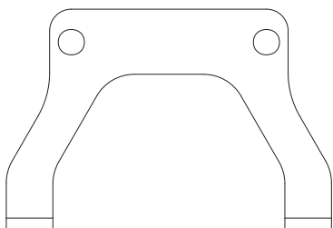
2. Shroud Bracket QTY 2
